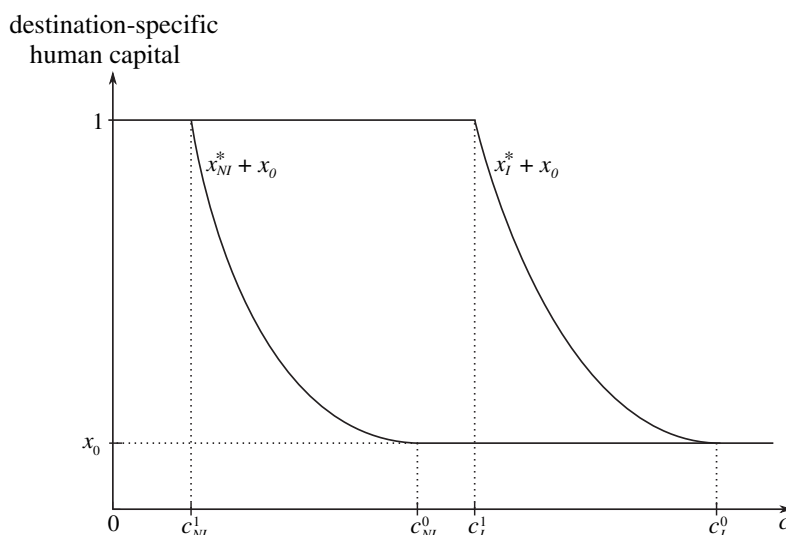
Fig. A1. x_{NI}^* + x_0 (the optimal level of destination-specific human capital of a non-integrated migrant), and x_I^* + x_0 (the optimal level of destination-specific human capital of an integrated migrant) as functions of the cost parameter c , for the utility function given in (A1), and for the case in which c_{NI}^0 \leq c_I^1 and c_I^0 < \infty .
