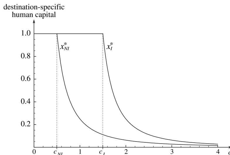
Fig. 1. x_{NI}^* (the optimal level of destination-specific human capital acquired by a non-integrated migrant), and x_I^* (the optimal level of destination-specific human capital acquired by an integrated migrant) as functions of the cost parameter c , for the utility function given in (8).
