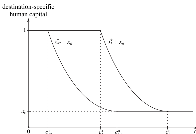
Fig. A2. x_{NI}^* + x_0 (the optimal level of destination-specific human capital of a non-integrated migrant), and x_I^* + x_0 (the optimal level of destination-specific human capital of an integrated migrant) as functions of the cost parameter c , for the utility function given in (A1), and for the case in which c_{NI}^0 > c_I^1 and c_I^0 < \infty .
