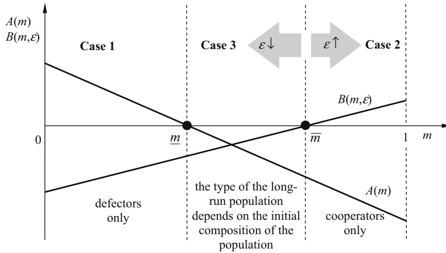
Fig. 1 A diagrammatic representation of A(m) and B(m, \epsilon) , and of the long-run composition of the population
